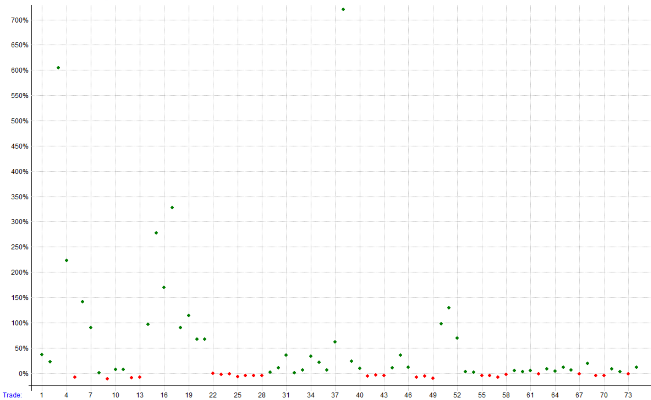
Test 14 - Combined - distribution of %gains
