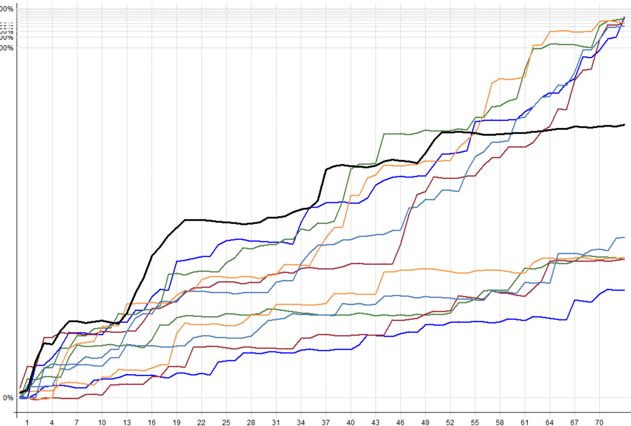
Test 14 - Combined - Monte Carlo %drawdown - 100 samples, showing worst 5
