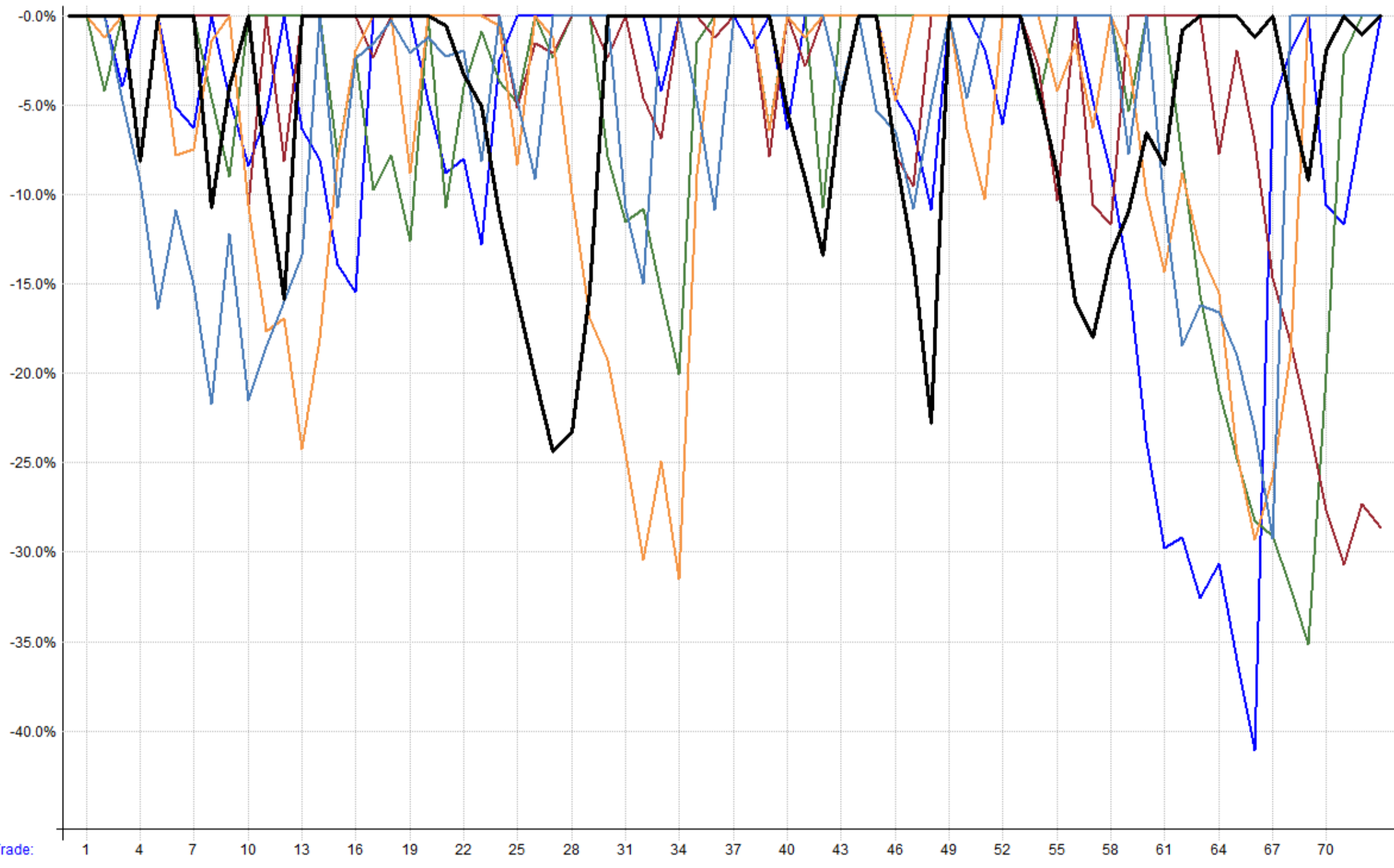
Test 14 - Combined - Monte Carlo %drawdown - 100 samples, showing worst 5
